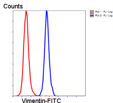
Fig. 4. Flow cytometric analysis of HeLa cells with Vimentin antibody at 1/50 dilution (blue) compared with an unlabelled control (cells without incubation with primary antibody; red). Goat anti mouse IgG
